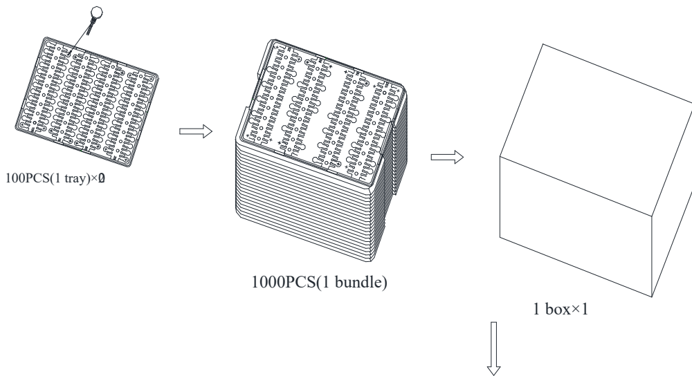
Pack drawing of coin type
